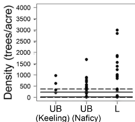
Figure 2. Total density in unlogged, unburned (UB) versus logged, unburned (L) sites relative to the observed range of variation in unlogged, repeatedly burned stands (two to four 20th century wildfires) for all species (A), ponderosa pine (B), Douglas-fir (C), and other species (D). Unlogged, unburned sites from Keeling et al. (2006) and Naficy et al. (2010) are shown separately. Solid lines represent the upper (75th percentile) and lower (25th) percentile bounds of the observed interquartile range for unlogged, repeatedly burned sites from Keeling et al. (2006), and dashed lines represent the upper (maximum) and lower (minimum) bounds of the full range of density values. The upper limits of the interquartile range and range for panel D were near 0 (5 and 20 trees acre -1 , respectively) because of the very low incidence of any species other than ponderosa pine and Douglas-fir in frequently burned sites.
